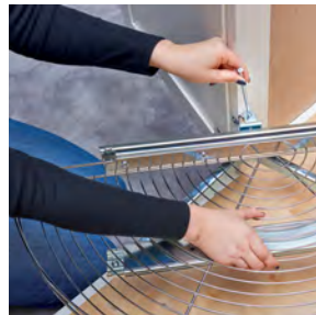
Chrome wire half moon Lazy Susan slide and pivot mechanism
